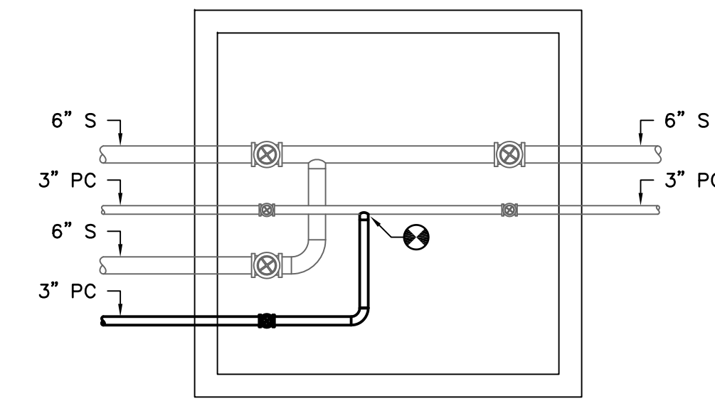
2 MANHOLE E5-3D NO SCALE
