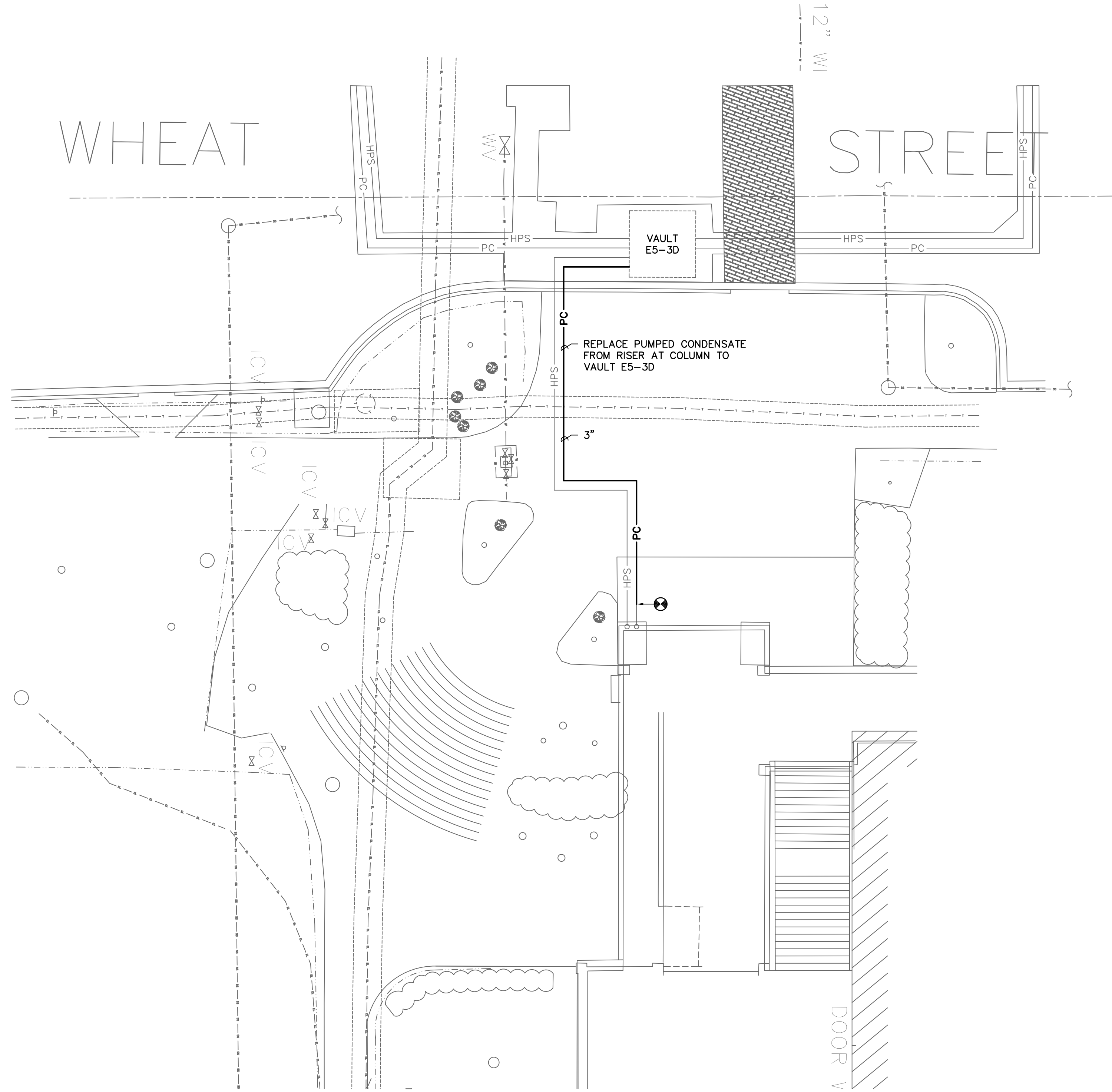
1 SITE PLAN - RENOVATION SCALE: 1" = 10'
